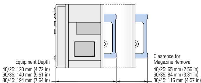
Allen Coding Compact Foll Models - Side Dimensions
