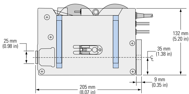
Allen Coding Compact Model 40/25
